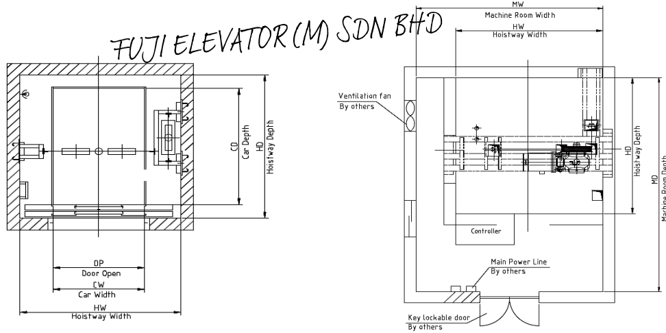
PLANNING GUIDE FOR DIMENSIONS OH and PIT-A100
