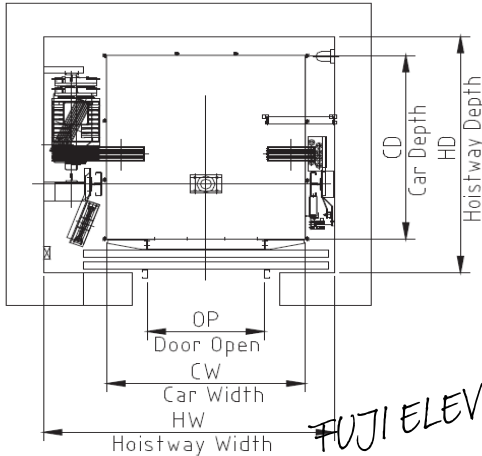
PLANNING GUIDE FOR DIMENSIONS 630-1050kg/ 1.0-1.75 mps
