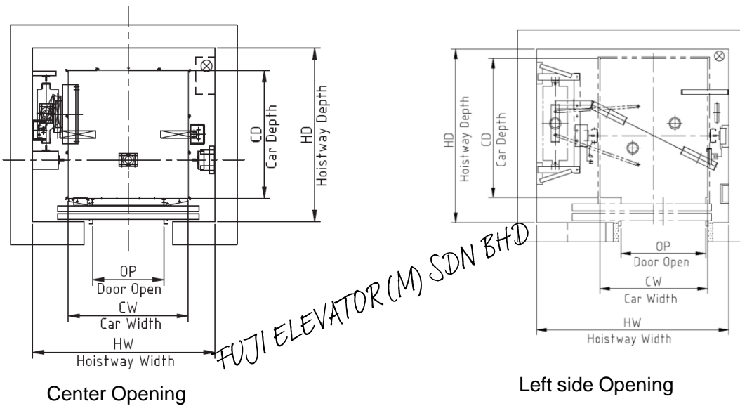
PLANNING GUIDE FOR DIMENSIONS -- Deep Car -- 630-1000kg
