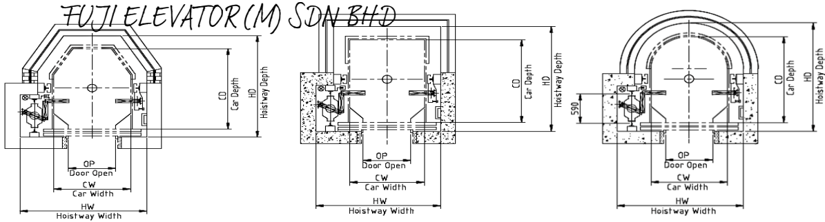
PLANNING GUIDE FOR DIMENSIONS -- Deep Car -- 630-1600kg
